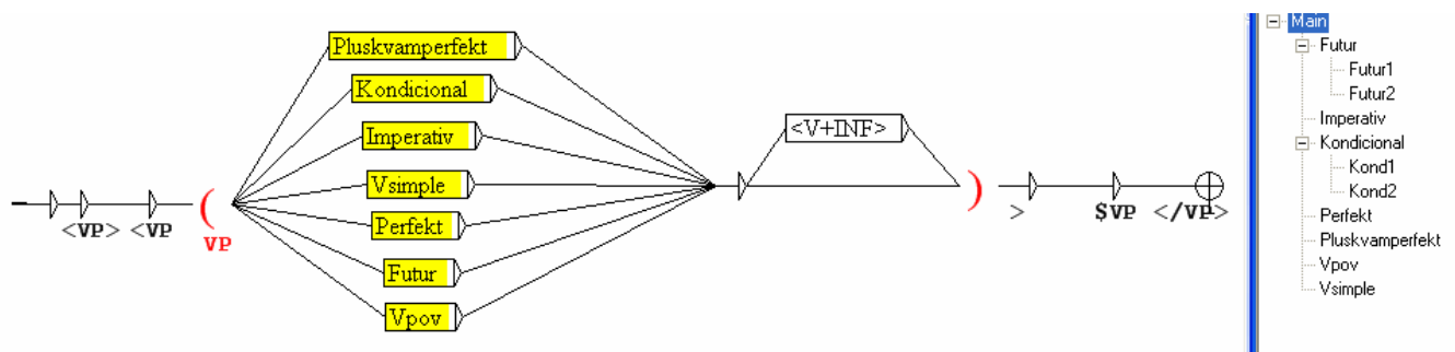
Figure 7. Graphical rendering of VP-chunk local grammar
