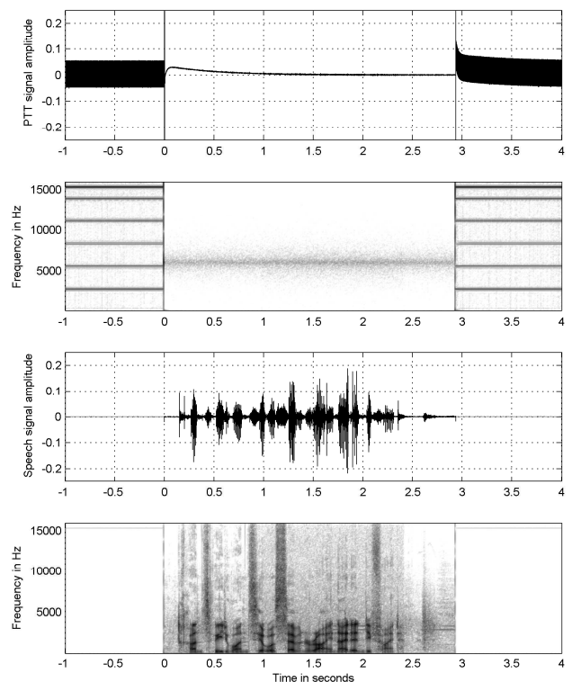
Figure 2: A short speech segment (transwede one zero seven rhein identified) with push-to-talk (PTT) signal. Time domain signal and spectrogram of the PTT signal (top two) and time-domain signal and spectrogram of the speech signal (bottom two)
