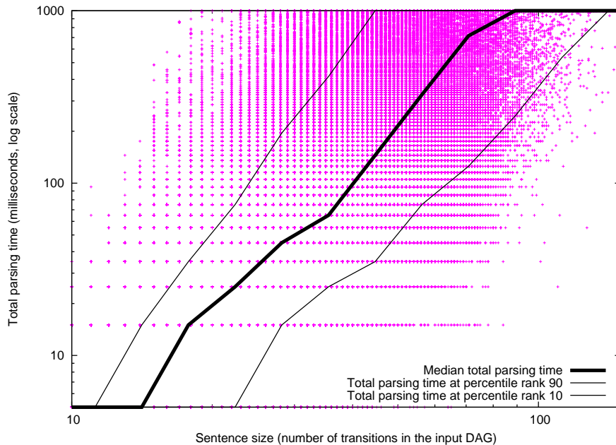
Figure 4: Total parsing time w.r.t. the length of the sentence (number of transitions in the input DAG of the sentence ; medians are computed on classes of sentences whose number of trees lies between 10^{2i} and 10^{2i+2} - 1 and plotted with a centered x -coordinate ( 10^{2i+1} )). See also footnote 4. Note that these results measure simultaneously the grammar's characteristics and SXLFG's performance.
