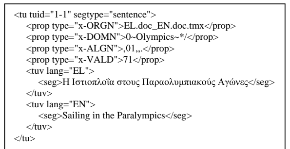
Figure 4. Example of Alignment Results in TMX
