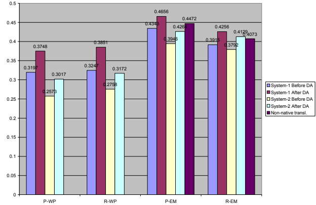
Figure 3. LTV scores – precision and recall
