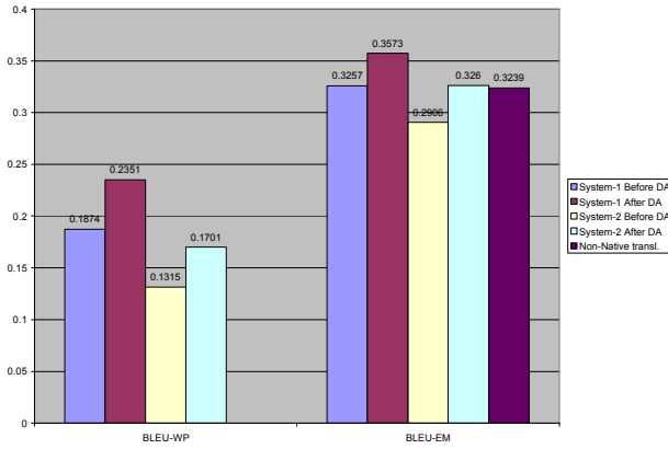
Figure 2. BLEU evaluation: usability and emails
