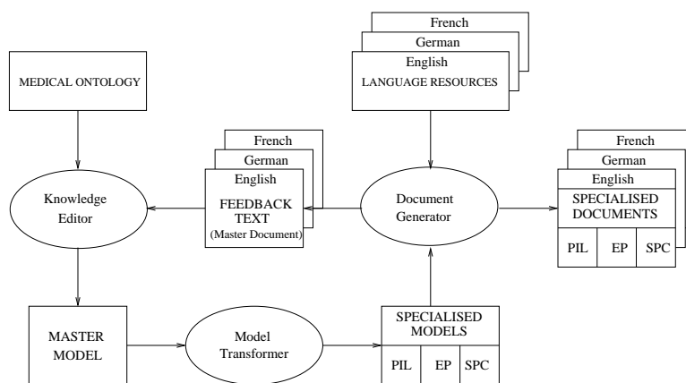
Figure 3: PILLS architecture
